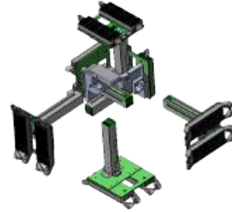
Fig. 6. Exploded view of prismatic module.
