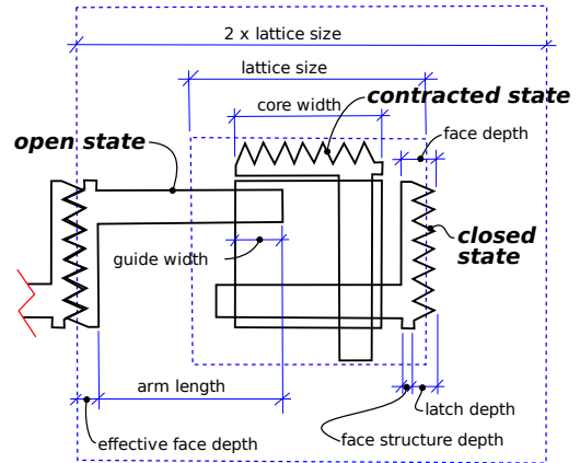
Fig. 7. Size and scaling parameters in the prismatic module design for the three states of a closed lattice system.
